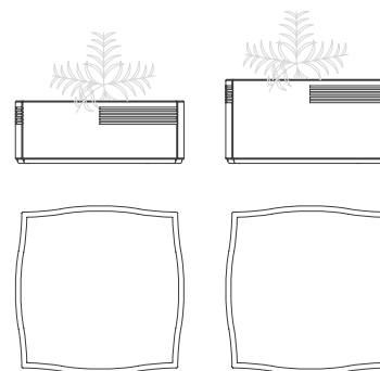
Fuat Q 60 | 162x162x60(h) cm | 1150 L Fuat Q 80 | 162x162x80(h) cm | 1570 L
